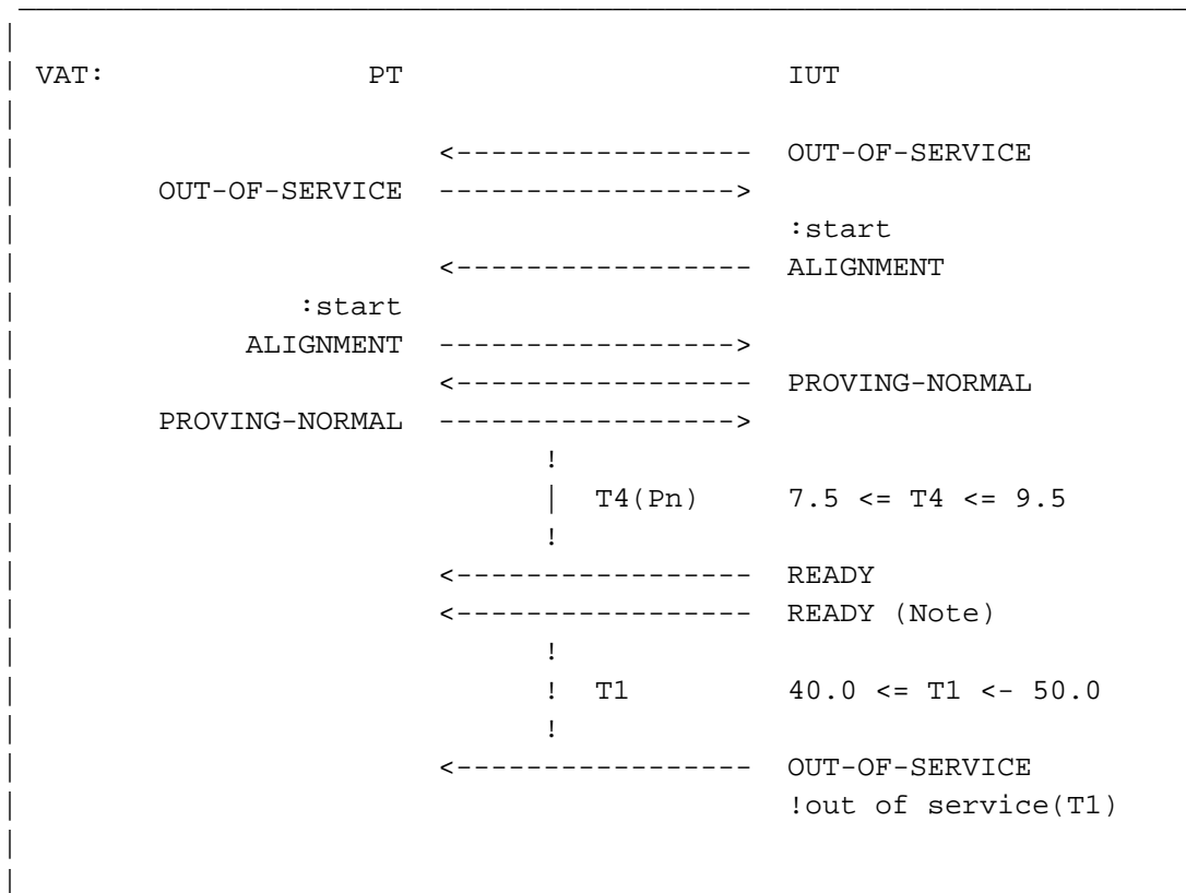
Figure 3.1.4-1. Timer T1 & Timer T4 (Normal)
