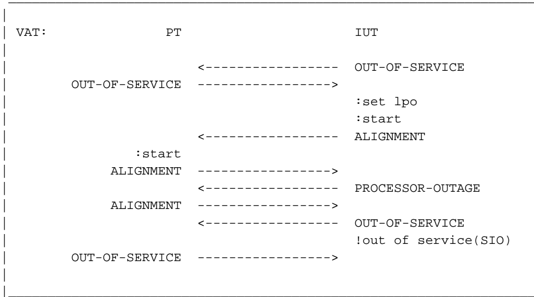
Figure 3.1.13-2. "Alignment" when "Aligned not ready"
