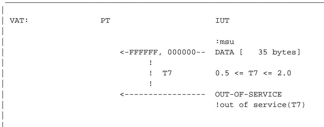
Figure 3.8.12-1. Excessive delay of acknowledgments
