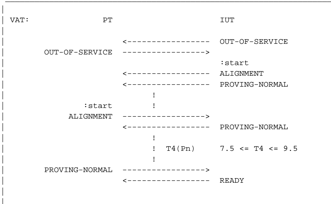
Figure 3.1.7-1. "Alignment" during normal proving
