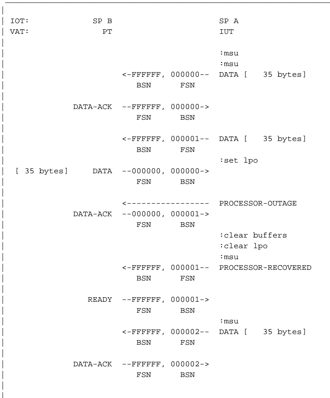
Figure 2.3.5-0 illustrates the labeling of sequence numbers. The Forward Sequence Number (FSN) is always labeled closest to the SP originating the message. The Backward Sequence Number (BSN) is always labeled closest to the SP receiving the message.
