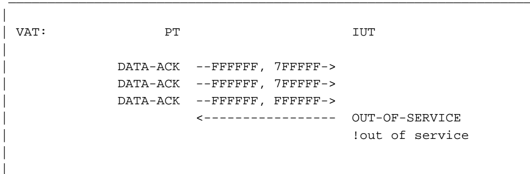
Figure 3.8.11-1. Abnormal BSN - two consecutive messages
