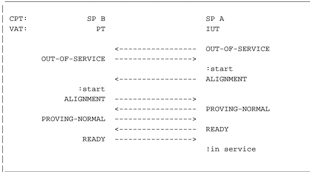
Figure 3.1.5-2. Normal alignment procedure
