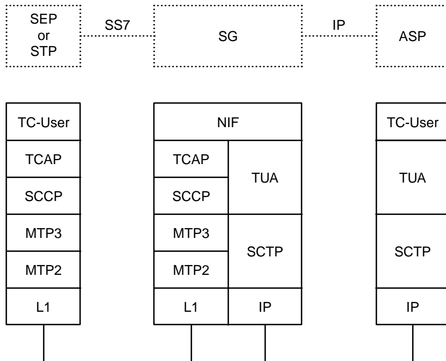
Figure 1. Protocol Architecture
